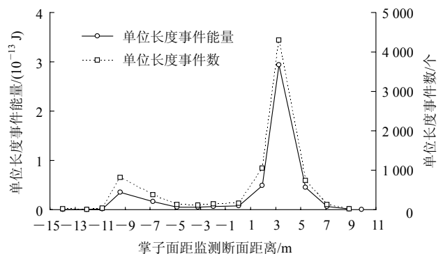
图 8 TBM 掘进时监测区域内声发射活动规律 Fig.8 Activity law of AE in monitoring zone during TBM excavation
