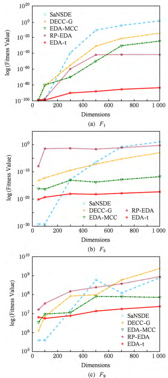
Fig. 4 Fitness value of five algorithms on different dimensions
