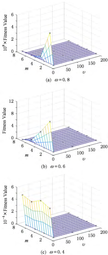
Fig. 5 Mesh grid of different parameters on functions F_5
