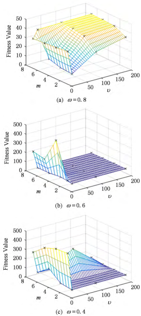
Fig. 6 Mesh grid of different parameters on functions F_7
