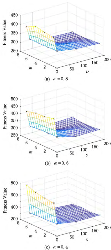
Fig. 7 Mesh grid of different parameters on functions F_{11}
