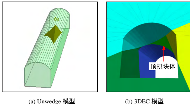
图 2 YB22 块体模型 Fig.2 Numerical models of YB22 block
