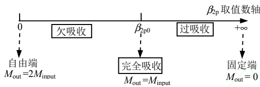
图 4 黏性吸收边界微调系数 \beta_{2p} 取值范围 Fig.4 The range of calibration factor \beta_{2p} for viscous boundary
