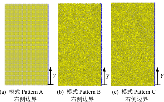
图10 计算模型右侧边界颗粒单元分布(蓝色线条) Fig.10 Distribution of particles on the right side of the model (the blue line)
