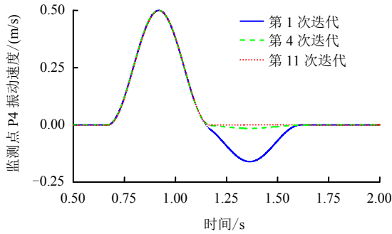
图8 \beta_{2p} 取2.0初值条件下, 监测点P4振动速度历程 Fig.8 The velocity history of P4 when \beta_{2p} takes 2.0
