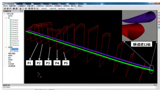
图 12 黄家寨隧道与各地质剖面模型 Fig.12 Models of geological sections and tunnels
