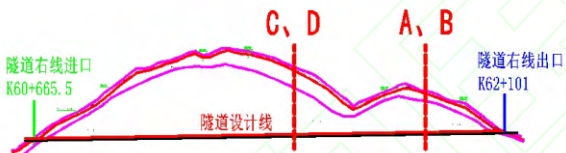
图 11 黄家寨隧道右线纵剖面图 Fig.11 Right line profile of Huang Jiazhai tunnel
