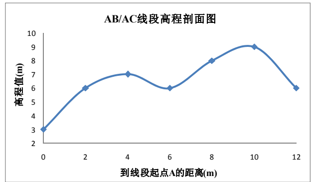
图4 AB/AC 线段高程剖面图 Fig.4 Elevation section map of segment of AC/AB
