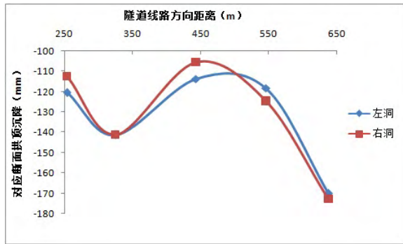
图 15 拱顶沉降曲线的计算 Fig.15 Crown settlement curves of different geological sections
