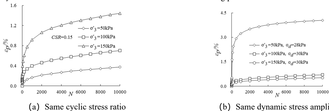
(a) Same cyclic stress ratio (b) Same dynamic stress amplitude Figure 5 Relationship between cumulative axial strain and vibration numbers under different consolidate confining pressures
