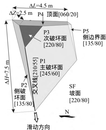
图 4 崩滑岩块体的三维几何描述 (平面产状: 倾向/倾角) [21] Fig.4 Three-dimensional geometrical representation of the collapsed rock wedge (plane orientatins: dip dir./dip) [21]
