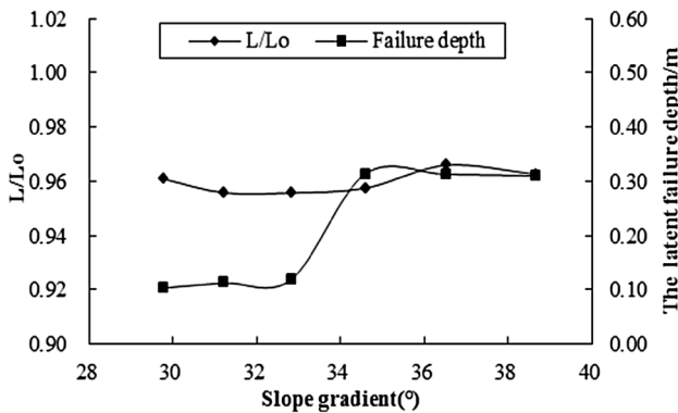
Fig. 8 Ratios of L to L_0 (failure length/total slope length), as well as the latent failure depth at section “1-1” versus gradient of slopes
