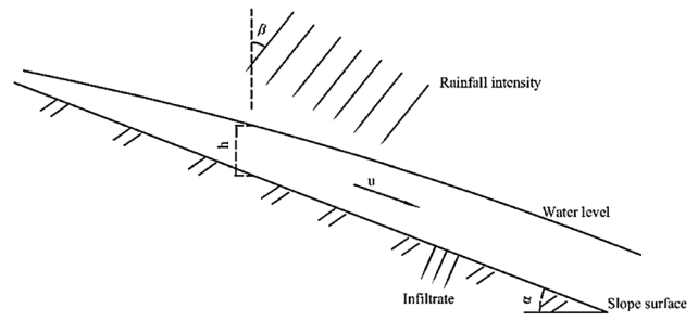
Fig. 1 Diagram of parameters in Saint–Venant equations, used to calculate slope infiltration
