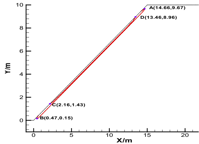
Fig. 5 Latent failure zones in slope when fluid–solid coupling is considered
