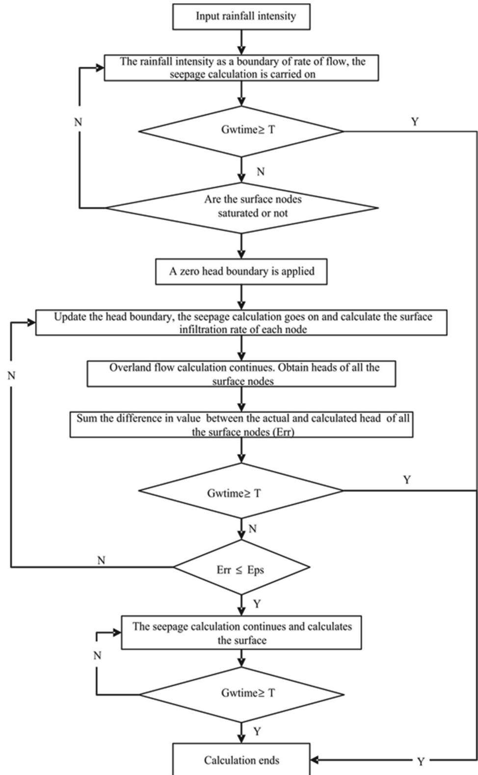
Fig. 2 Flow chart of coupling model of the surface–subsurface flows
