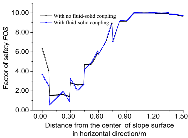
Fig. 6 Distribution of FOS versus the horizontal failure depth away from the slope surface in Section “1-1” (in Fig. 3)
