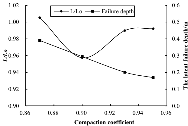
Fig. 13 Ratio of L to L_0 , and failure depth versus compaction coefficient
