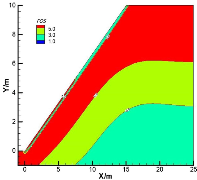
Fig. 4 Distribution map of FOS for slope when fluid–solid coupling is not considered
