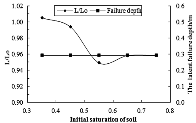
Fig. 12 Ratio of L to L_0 , and failure depth versus initial soil saturation
