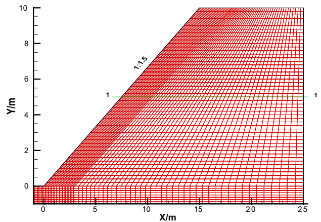
Fig. 3 Finite element grid model, here “1-1” is a horizontal section
