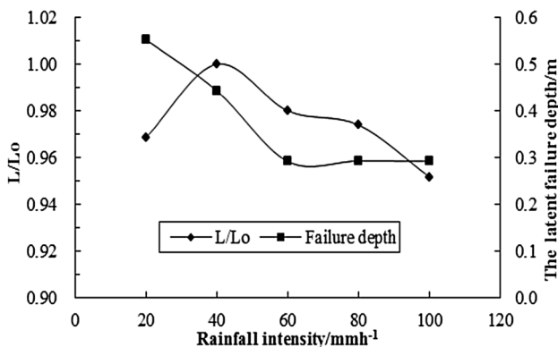
Fig. 11 Ratio of L to L_0 , and failure depth versus rainfall intensity, and the total rainfall remains constant
