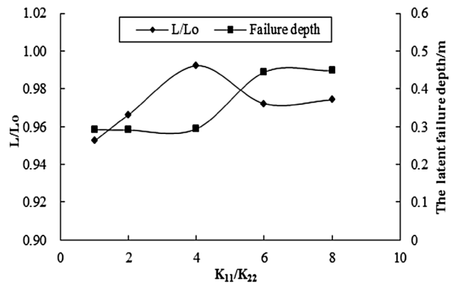
Fig. 10 Ratios of L to L_0 , as well as the latent failure depth at section “1-1” versus ratios of K_{11} to K_{22}
